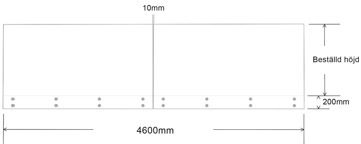
8st FixPoints - maxbredd glas 2300mm
